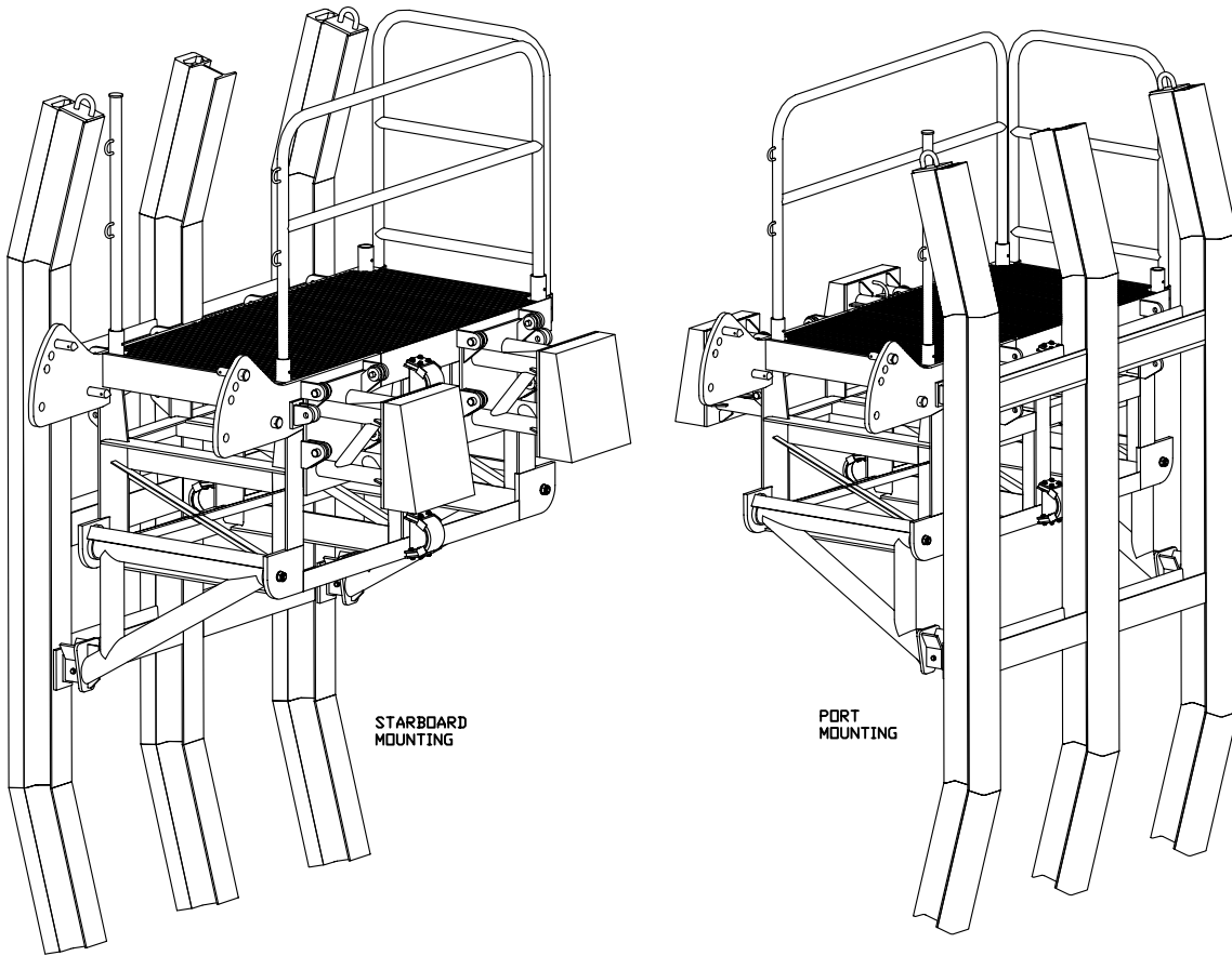
LOWER PLATFORM SHOWN WITH BOAT FENDER & SHELL BUMPERS
