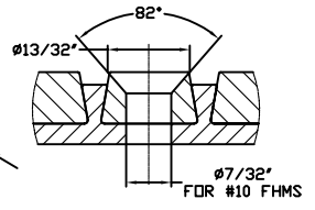
DETAIL B (TYPICAL)
